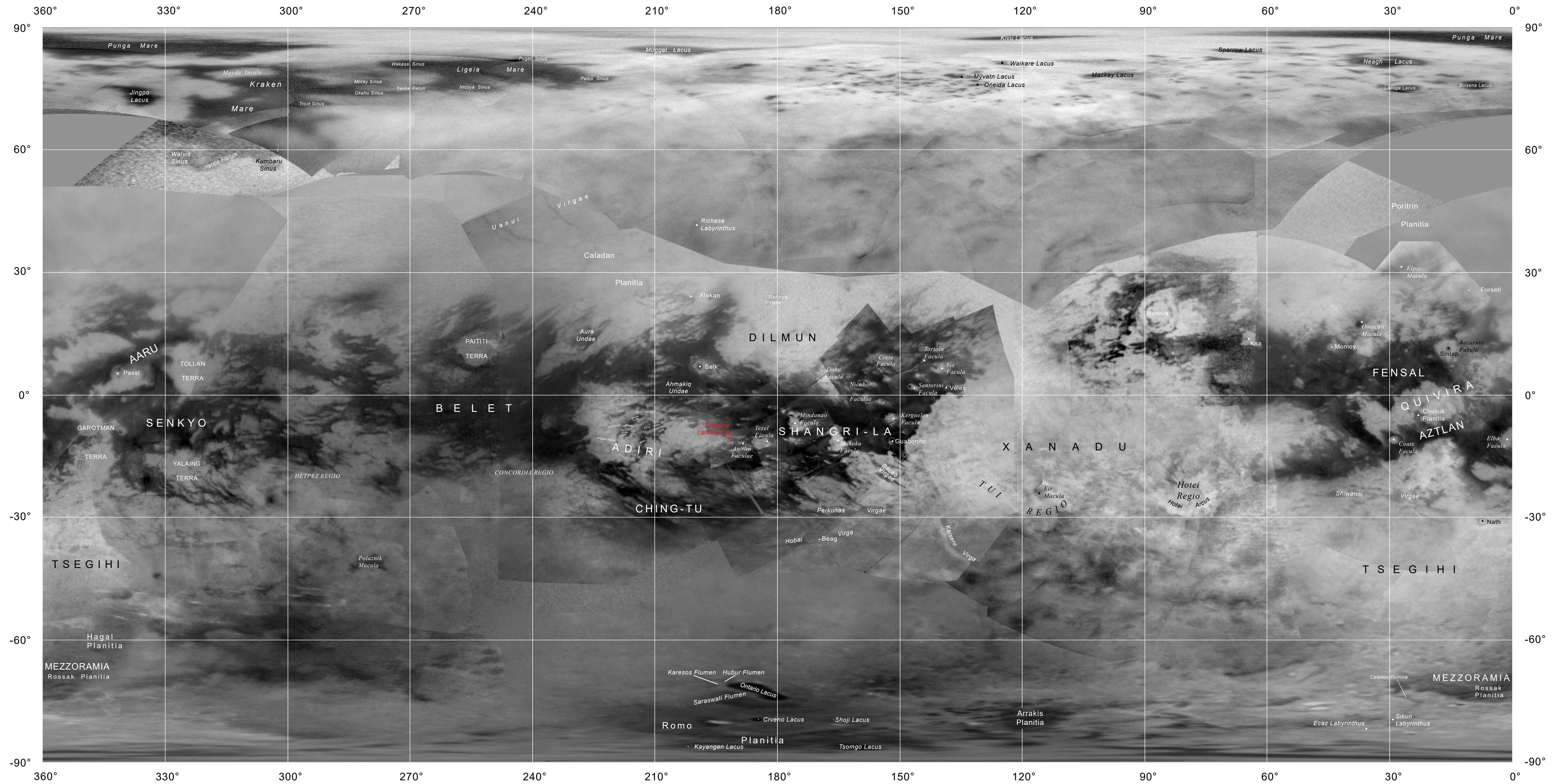
Basemap: Cassini ISS Global Mosaic
